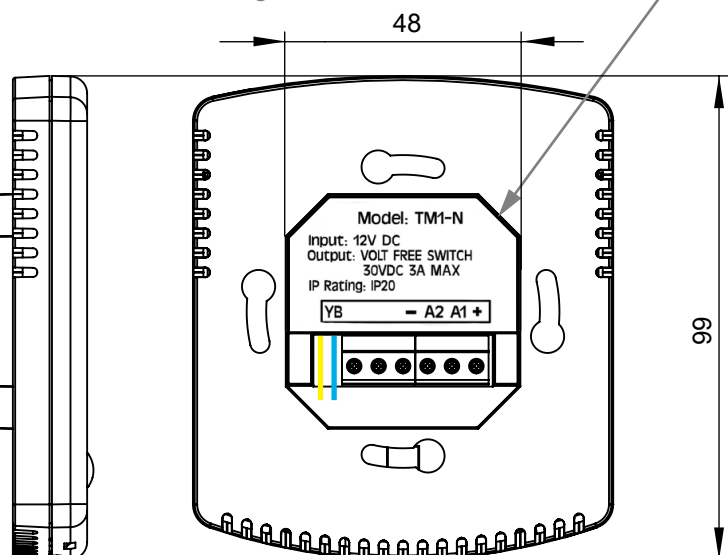
Wiring Detail
