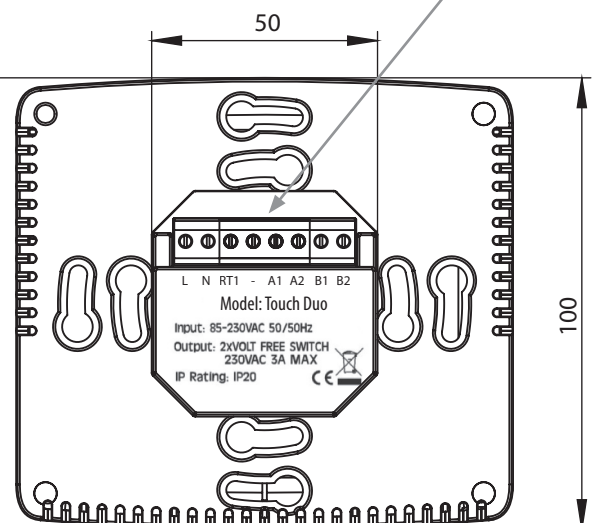
Wiring Detail
