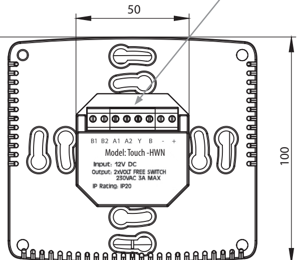
Wiring Detail
